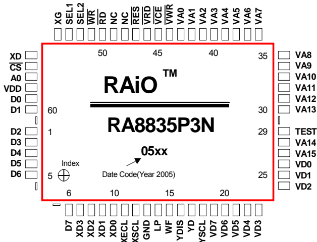
Figure 4-1: RA8835P3N(QFP-60 Pin)
